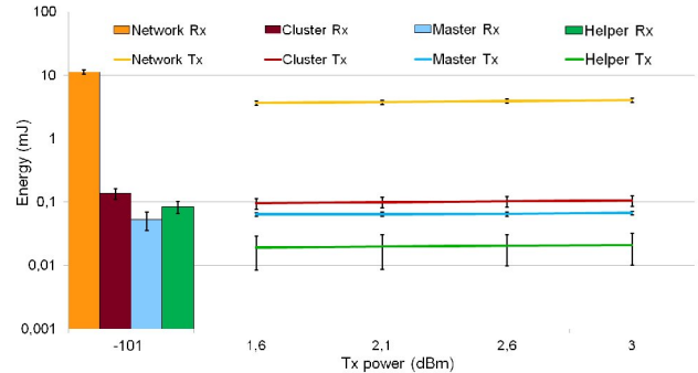
Figure 3: Mean and stdev of energy consumed for Rx and for Tx operations (as a function of the node's Tx power). Network and Cluster-level analysis for the 100 nodes scenario.
