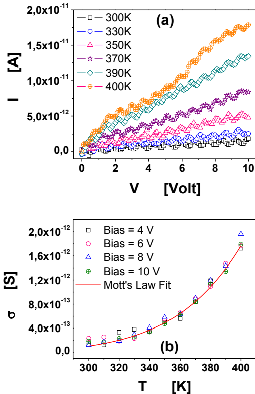
Fig. 2. (a) Current-Voltage characteristics for different temperatures and (b) Temperature dependence of AlN conductivity revealing Mott's law.
