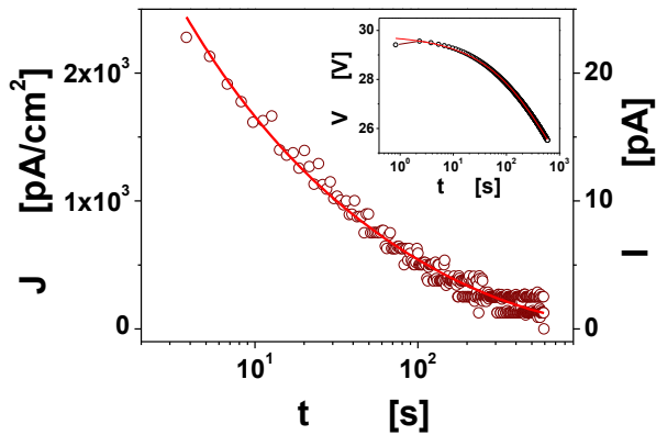
Fig. 4. Bulk discharge current calculated after stressing the device at 12 pA. The inset graph presents the decay of potential during the depolarization process. Solid lines represent the fitting of data with Eqs.9 and 11.
