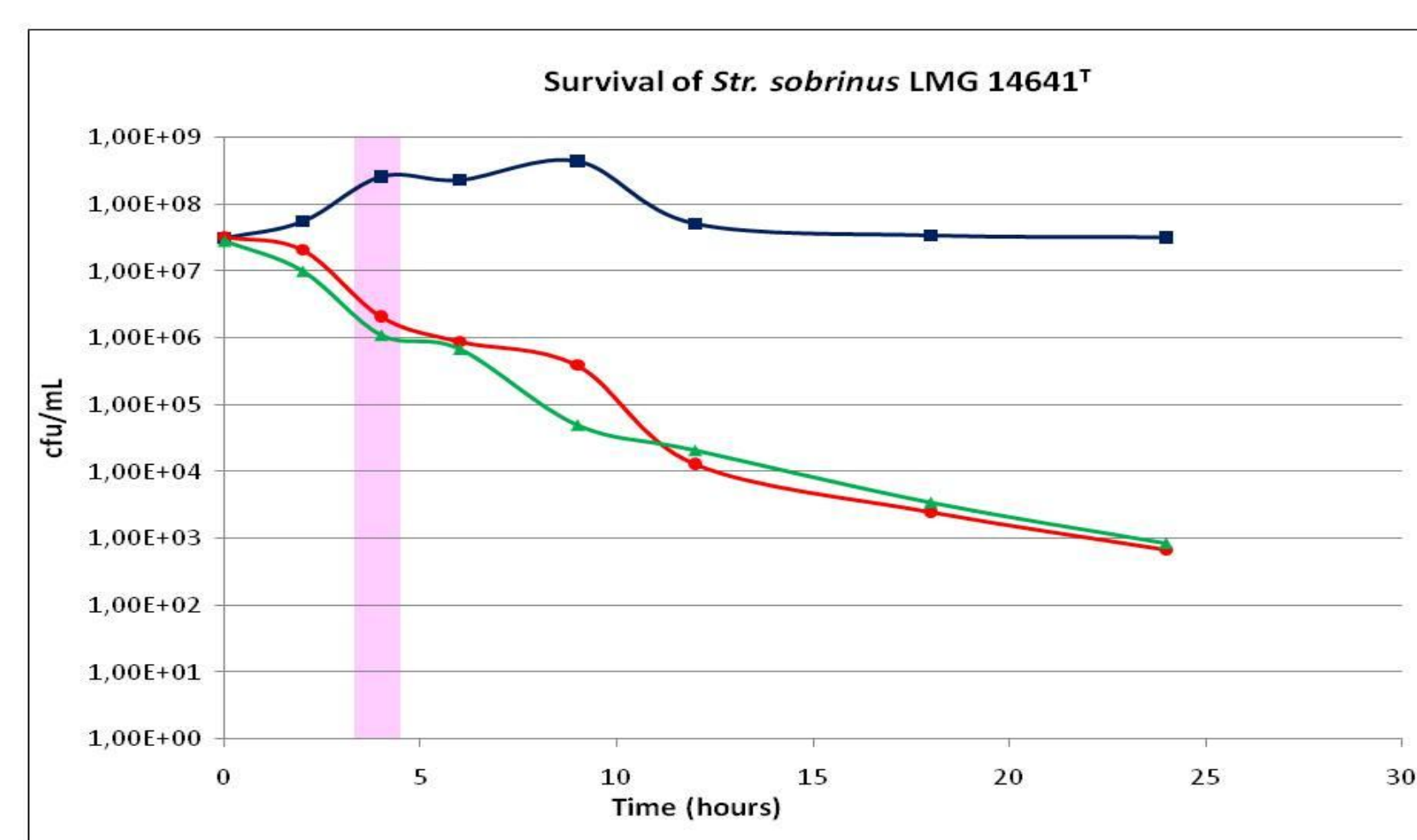
Figure 2. Time killing studies of logarithmic cells of Str. mutans LMG 14558, Str. oralis LMG 14532 and Str. sobrinus LMG 14641 after their incubation with the control sample (MeOH 70%) (●); 28 mg/mL methanolic extract of Crocus sativus L. (●); 28 mg/mL methanolic extract of Melissa officinalis L. (▲).
