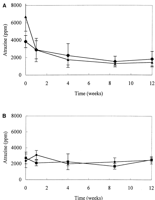
Fig. 2. Atrazine biodegradation in field test plots. A. (◆) Bioaugmentation plots (0.5% killed recombinant E. coli cells) and (▲) biostimulation plus bioaugmentation plots (0.5% killed recombinant E. coli cells plus 300 p.p.m. phosphate). B. (●) Control and (■) biostimulation (300 p.p.m. phosphate) plots. Error bars represent 1 standard deviation. Soil temperature over the experimental time period at 10 cm depth dropped from 19.2°C to 3.6°C.
